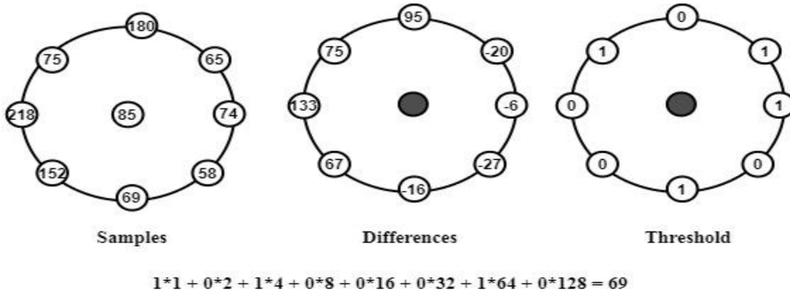
Figure 6: Computation level of LBP in machine learning
