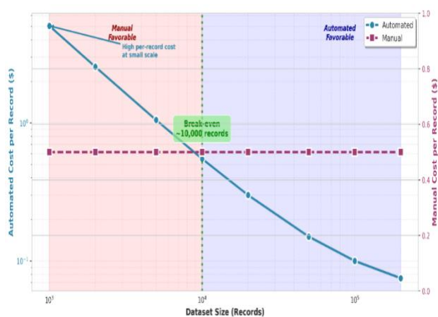
Figure 7: Cost per record across dataset scales with break-even threshold.
