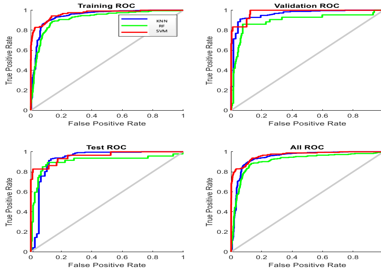
Figure 8: Comparison of ROC curves for the SVM, KNN, and RF classifiers in hand gesture recognition using sparse transform features after feature selection.
