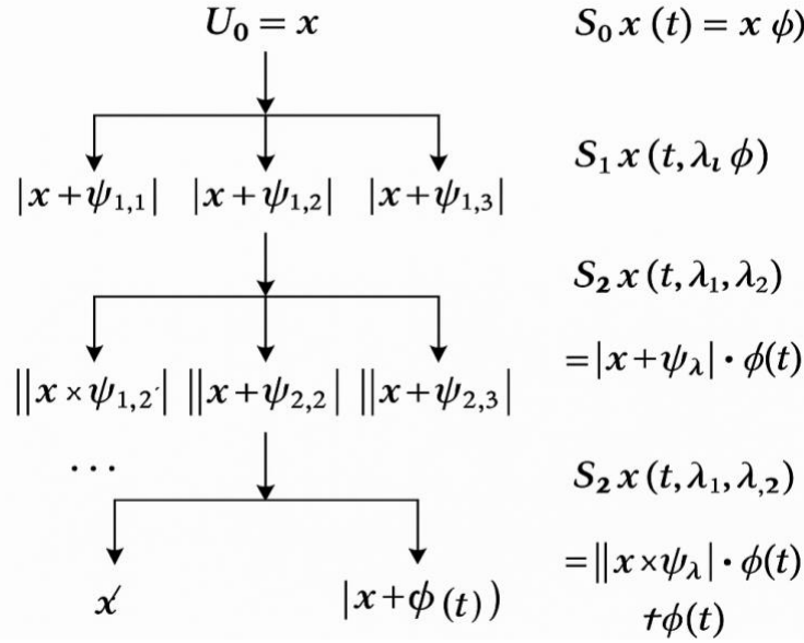
Figure 4: Coefficient calculation in the subsequent layers of the transform.
