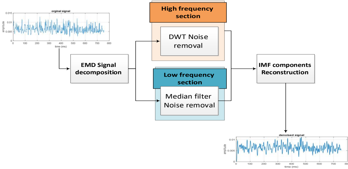
Figure 2: Preprocessing process in the proposed method
