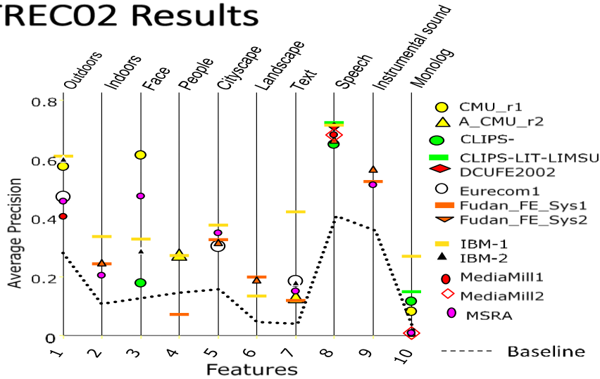
Figure 6: TRECVID 2002 feature extraction results (adapted from [5])
