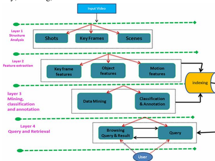
Figure 2: Content Based Video Retrieval (CBVR) model (adapted from [31])
