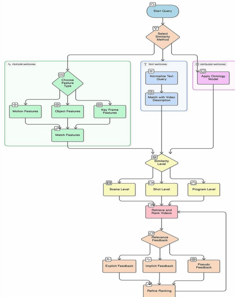
Figure 4: Relevance feedback block diagram
