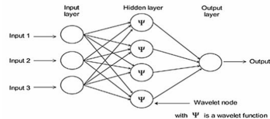
D) Structure of a WNN
