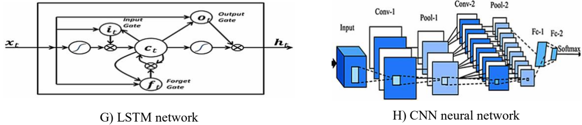
Figure 2: Types of deep neural networks
