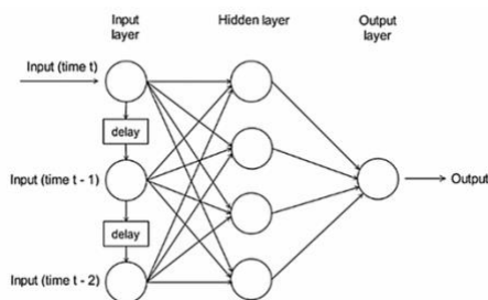
E) TDNN neural networks
