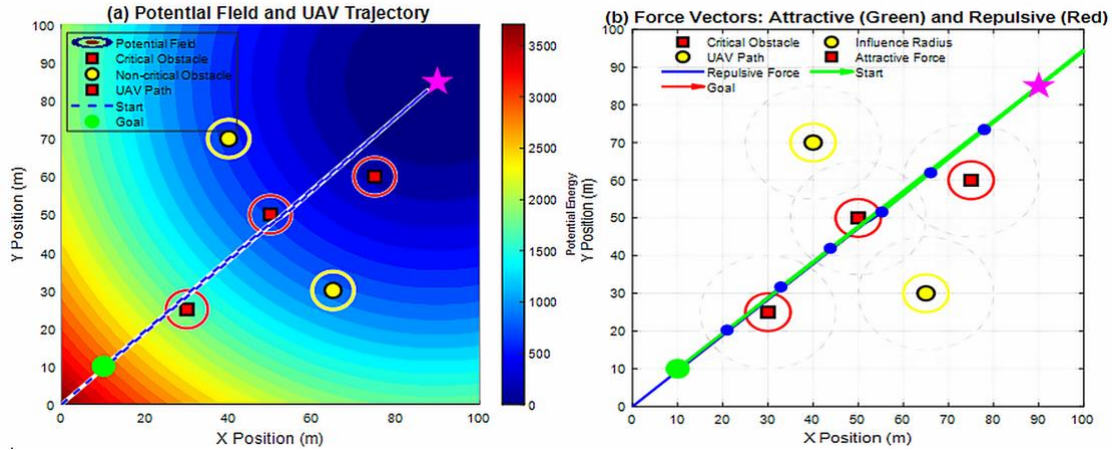
Figure 3: Potential field-based navigation showing repulsive forces from detected obstacles and attractive force toward the goal position.
