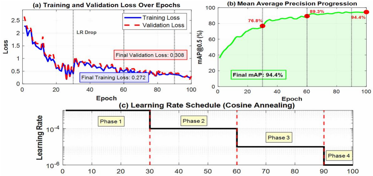
Figure 6: Training convergence curves showing loss reduction and mAP improvement over 100 training epochs.
