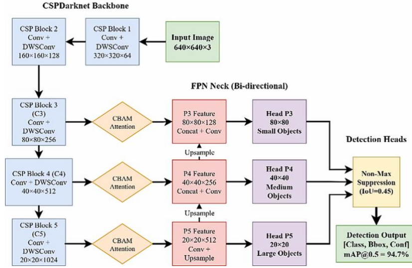
Figure 2: Modified YOLO architecture with spatial attention mechanism for aerial object detection.
