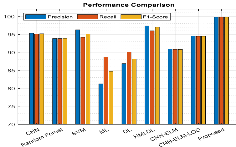
Figure 9: An evaluation of the proposed method in relation to previous studies is presented, using precision, recall, and F1-score.
