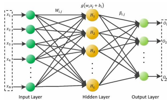
Figure 5: General structure of the ELM.
