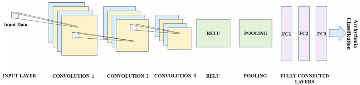
Figure 4: Structure of the proposed CNN.
