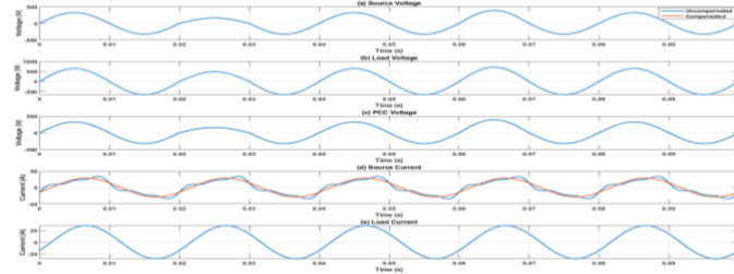
Figure 3: waveform for one Pareto optimal solutions.
